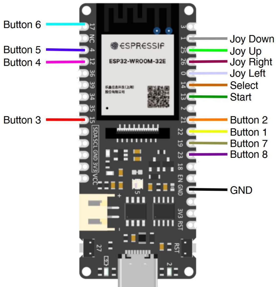
Picture 48 - ESP32-E (N16R2) DFR1139 proposed connection diagram
