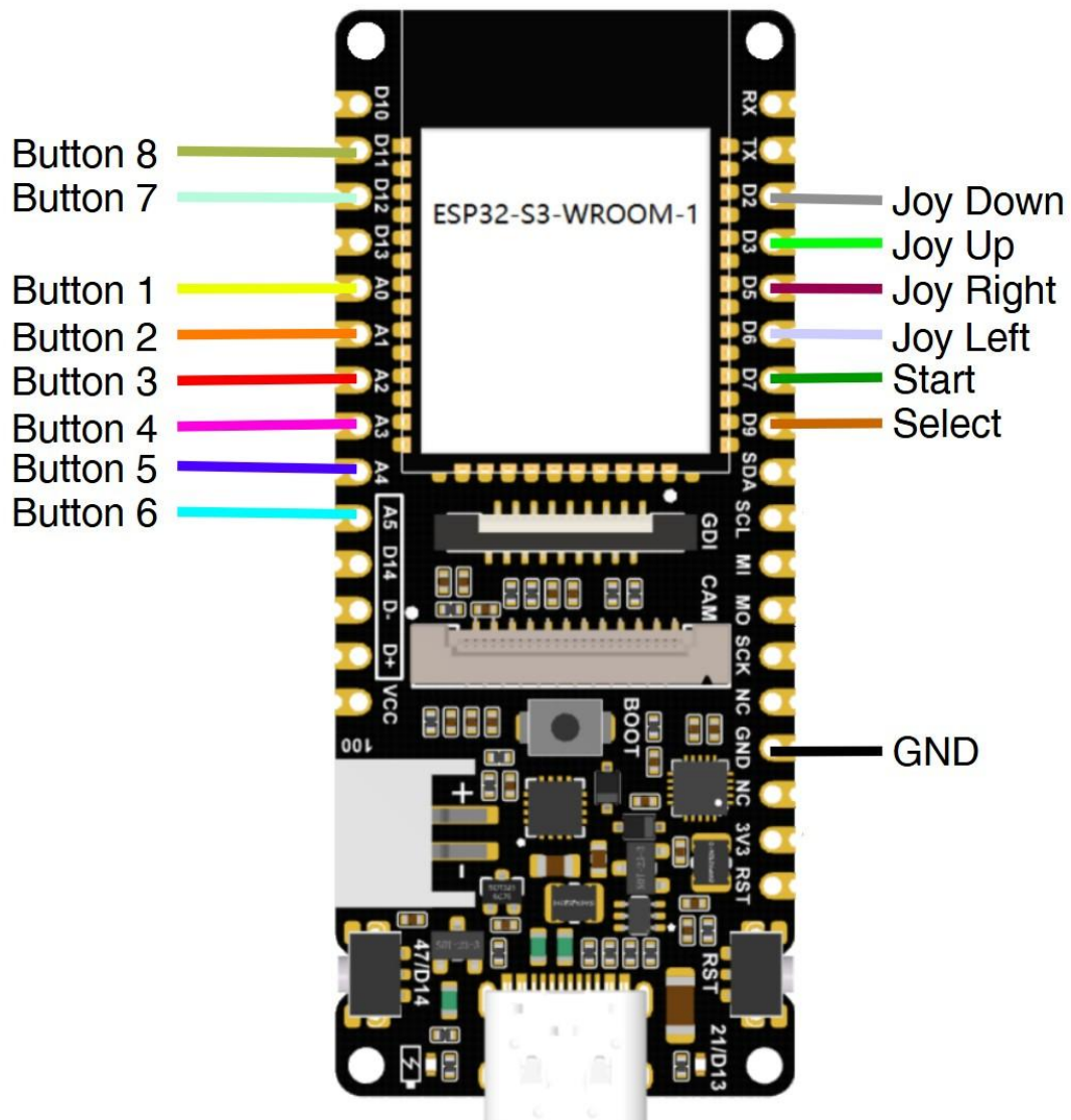
Picture 47 - ESP32-S3 DFR1145 proposed connection diagram
