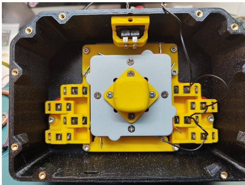
Picture 41 – daisy chaining the GND
