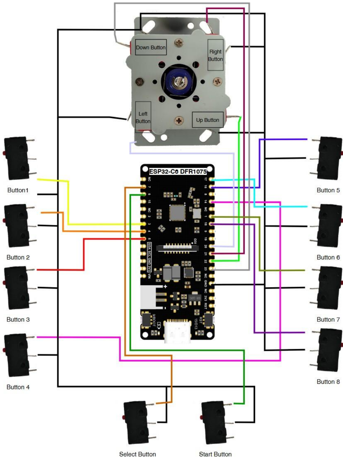
Picture 45 - Wiring Diagram for the ESP32-C6
